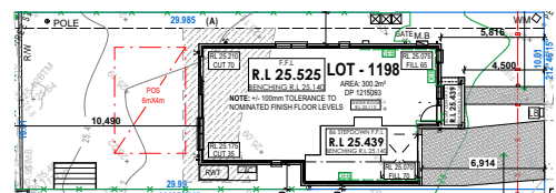
SITE PLAN
